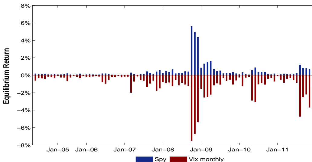
Figure 10 Equilibrium Returns
